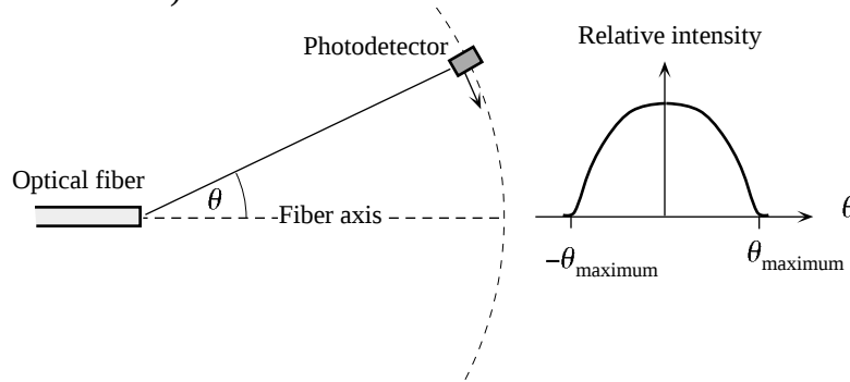
Far field distribuion from an optical fiber
